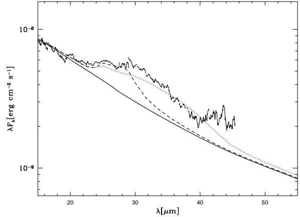
Fig. 2. Fitting to the 30 micron emission. The thin solid line is the ISO-SWS spectrum and the thick line stands for the model fitting result to spectral energy distribution, the same as in Fig.1. The dot and dash lines represent the fitting by assuming the CDE and Mie approximation for the computation of optical properties of the MgS grains, respectively; n(\text{S})/n(\text{H}) = 3.0 \times 10^{-6} .
